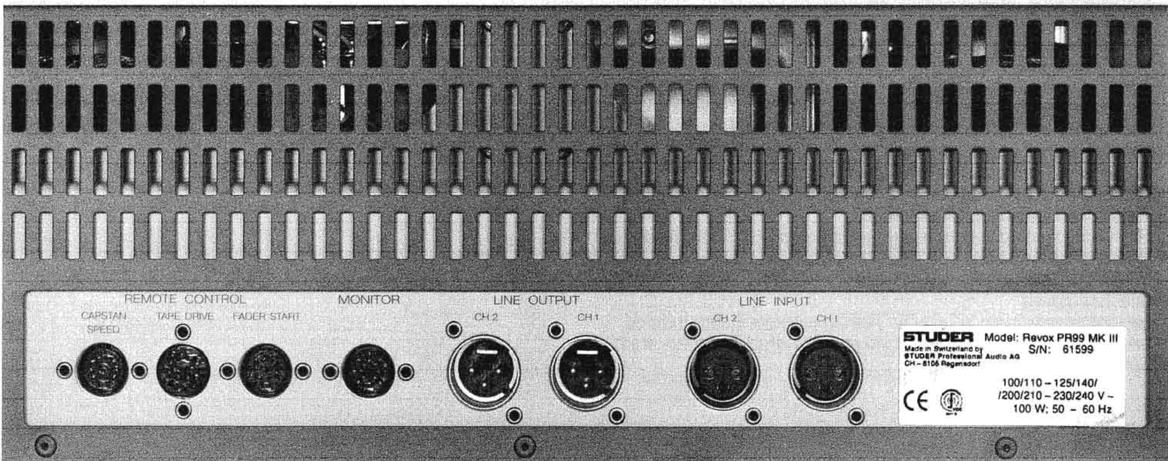
External capstan control
