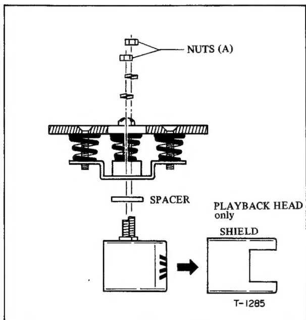
Fig. 6-1 Head Replacement
